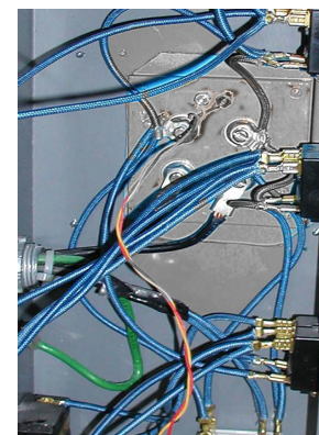
Connect wires to back of Electro Sitter just like the connections to the back of the kiln sitter.
